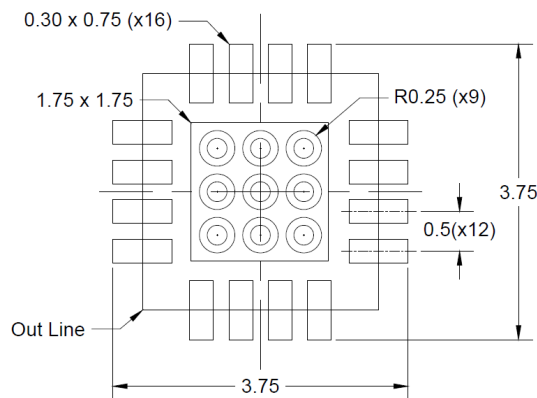
Figure 22 Recommended Land Pattern
