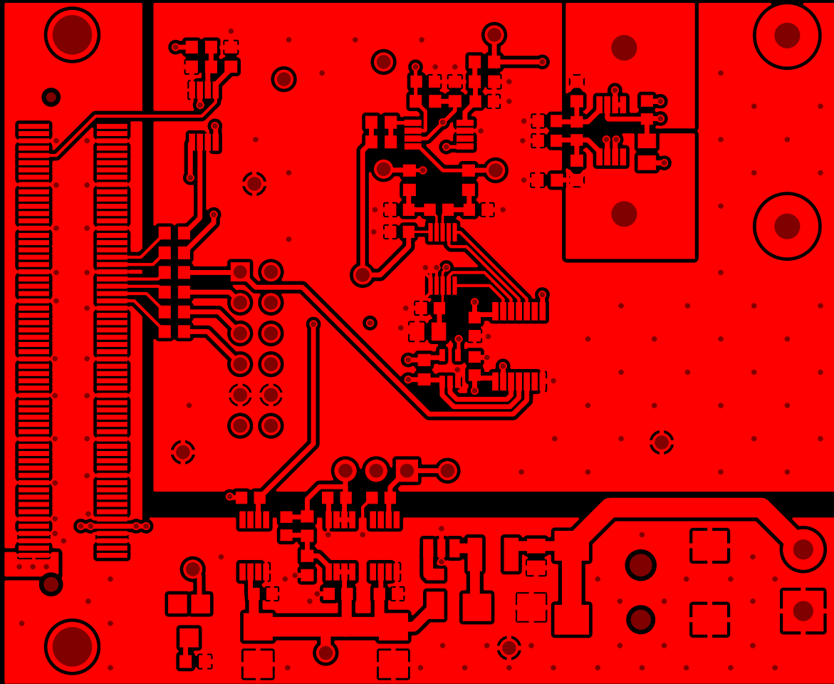
Top Copper
