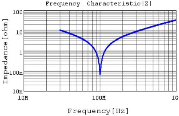
RCE5C2E471J1K1H03B |Z| DC0V, 25degC
