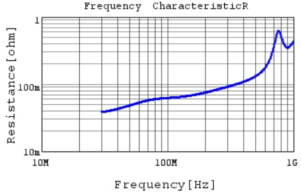
RCE5C2E471J1K1H03B R DC0V, 25degC
