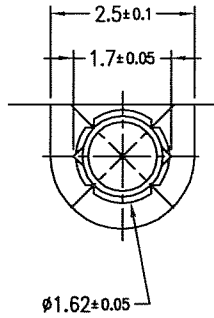
DETAIL "A" S=16/1
