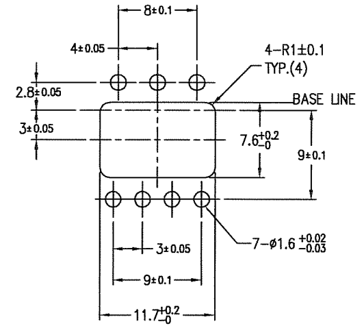
RECOMMENDED FOOT PATTERN
