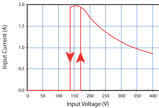
INPUT CHARACTERISTIC, I_{out} = 11.0A, T_c=25^\circ C
