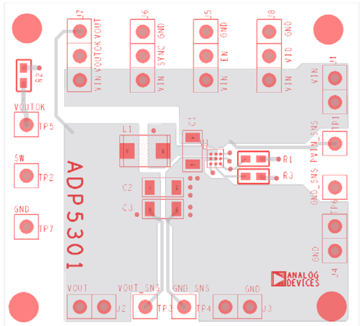
Figure 4. Top Layer
