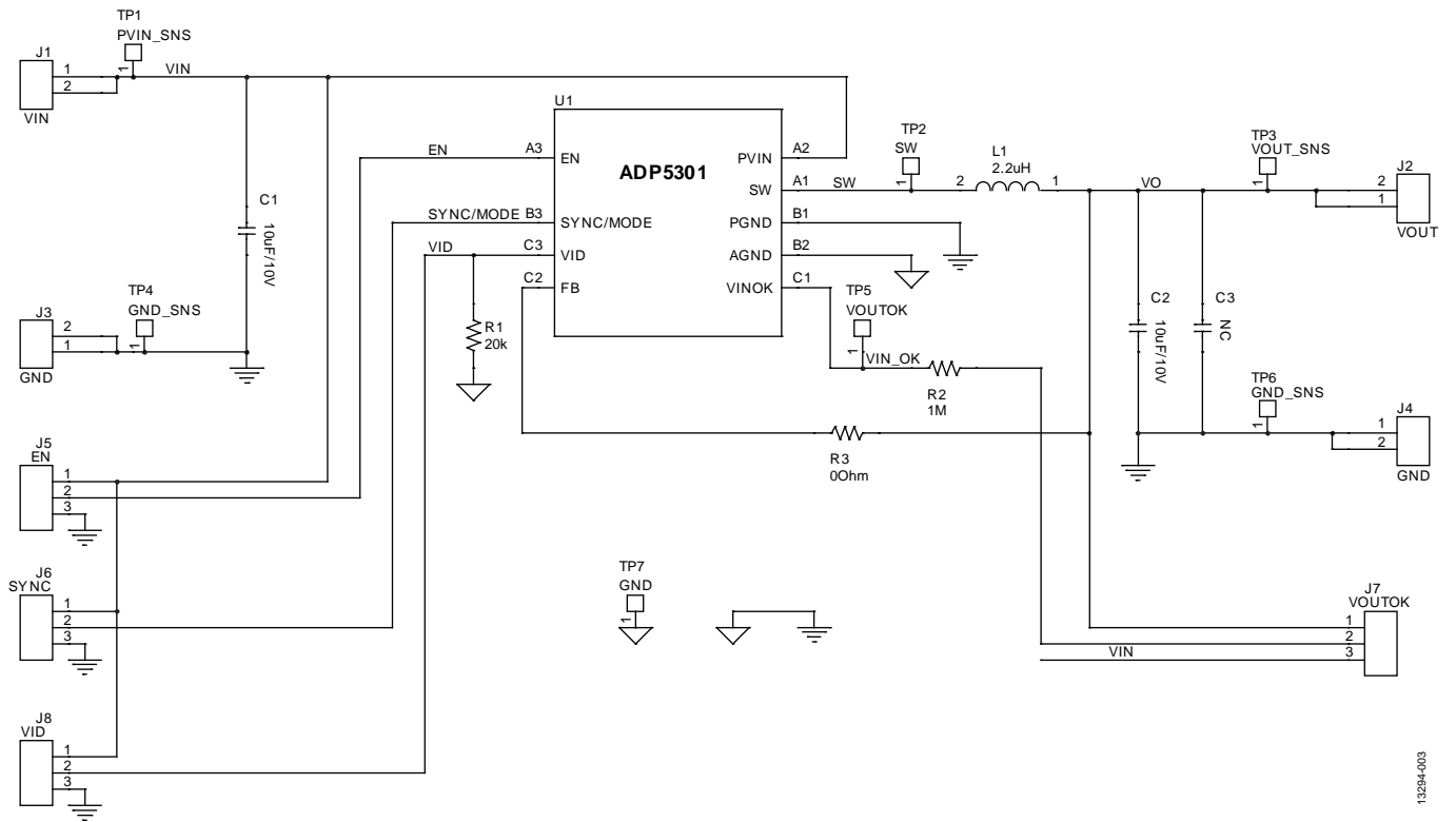
Figure 3. Schematic of the ADP5301-EVALZ Evaluation Board
