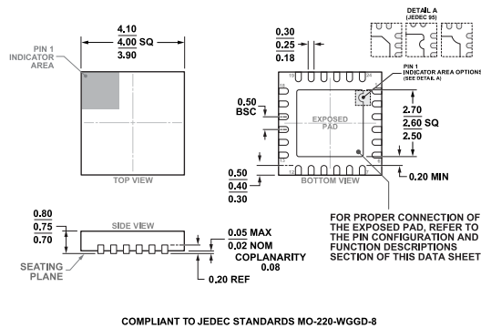
Figure 45. 24-Lead Lead-frame Chip Scale Package [LFCSP] 4 mm x 4 mm and 0.75 mm Package Height (CP-24-15) Dimensions shown in millimeters
