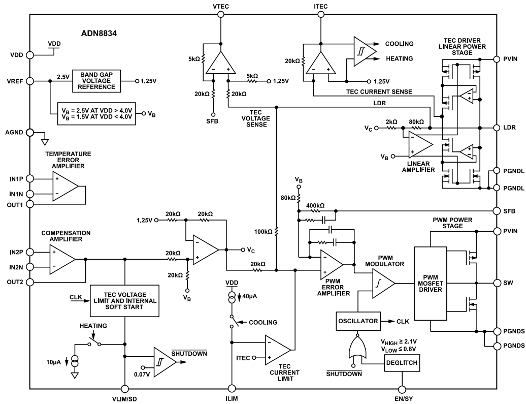
Figure 25. Detailed Functional Block Diagram of the ADN8834 for the WLCSPP
