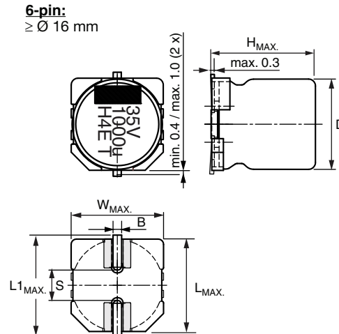
Fig. 1 - Dimensional outline
