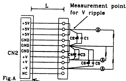
Fig.A L: 150mm AWG#18 C1,C3,C5:Film Cap 0.1µF C2,C4,C6:Elec.Cap 100µF Measurement point for Vo Load/Line regulation
