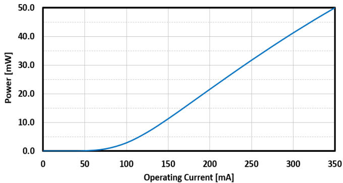
FIG. 11: SLED 4 OUTPUT POWER VS CURRENT
