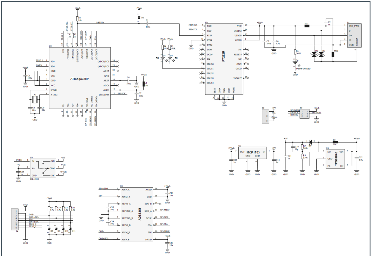
Figure 7: AS5715_BP_x.x Schematic
