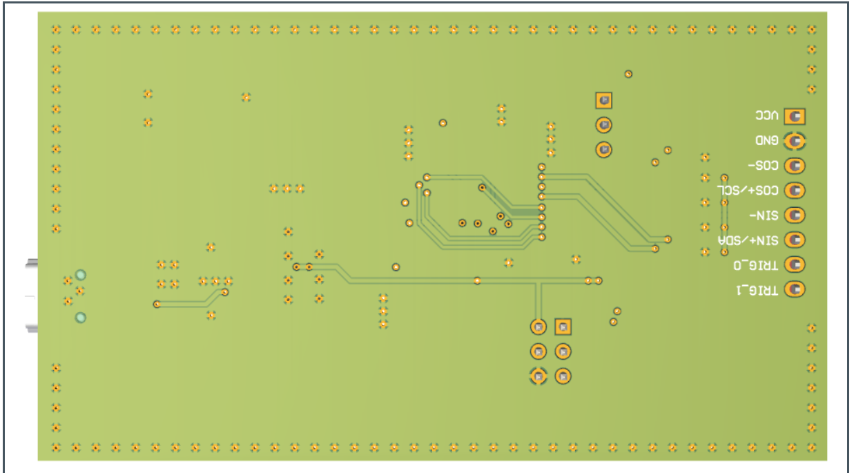
Figure 4: AS5715_BP_x.x Bottom View
