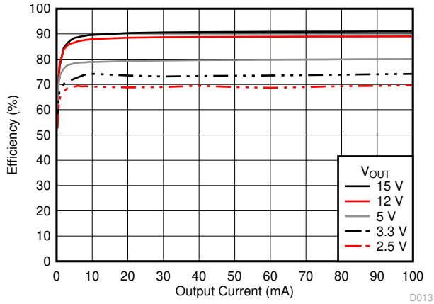
Figure 6-11. Efficiency
