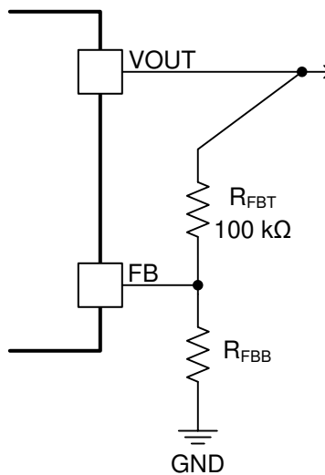
Figure 7-1. FB Resistor Divider
