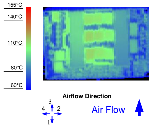
Figure 10. Thermal Image for Airflow Direction 3 (86.5A output, 55°C ambient, 200 LFM, typical V_{in} , open frame, soldered interface)
