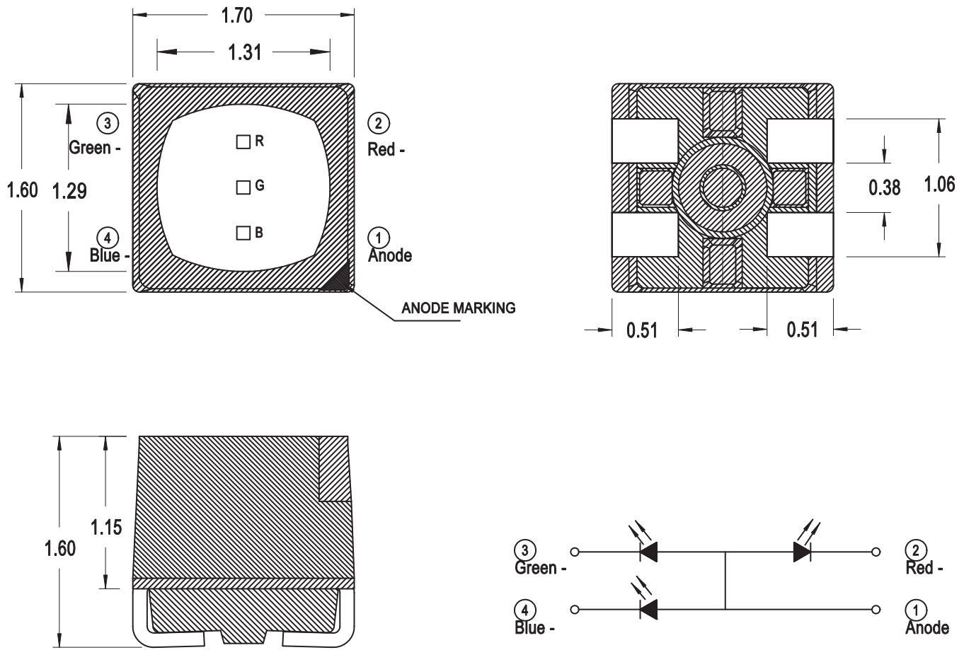
Figure 1: Package Drawing
