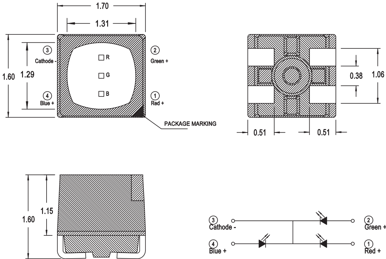
Figure 2: Package Drawing
