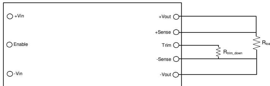
Figure 16. Trim DOWN circuit configuration
