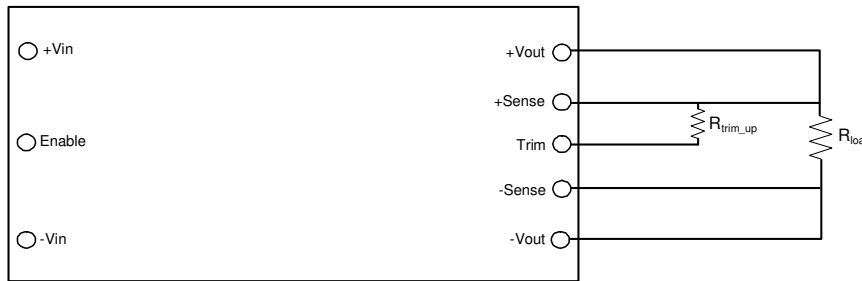
Figure 15. Trim UP circuit configuration
