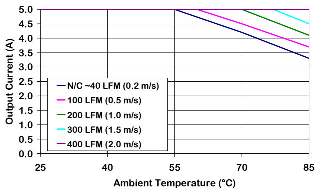
Figure 6. Output Current Derating vs Ambient Temperature & Airflow (converter mounted vertically with air flowing from pin 1 to pin 3, Vin = 48 V.)
