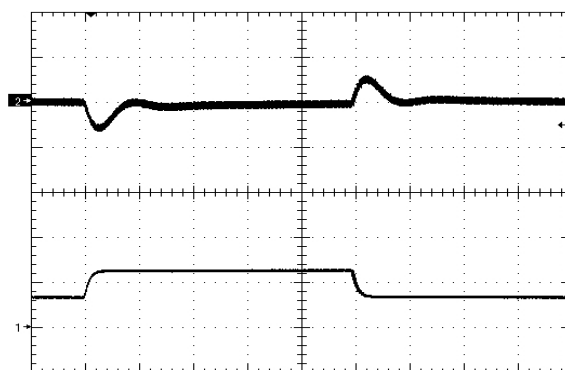
Figure 14. Load Transient Response (100mV/div), di/dt=0.1A/uS, 25% - 50% - 25% of full load, 440uF electrolytic across output, time scale: 200uS/div.
