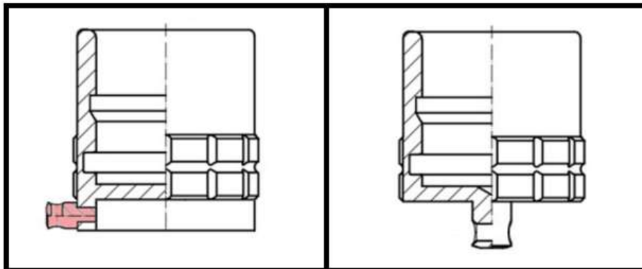
Previous Design 2-piece
