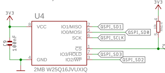
Flash memory
