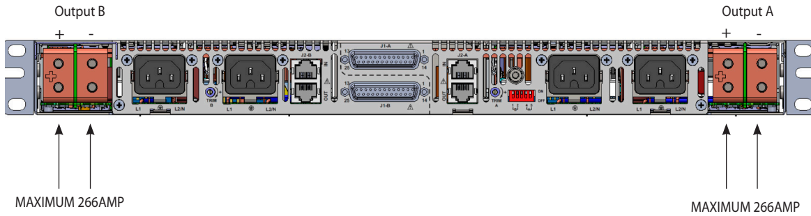
Fig 1.3a Output Bus-Bars.
