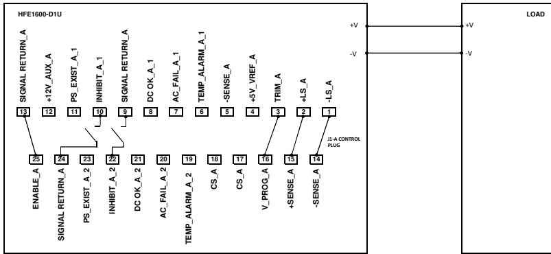
Fig 3.4 individual units On/Off diagram.
