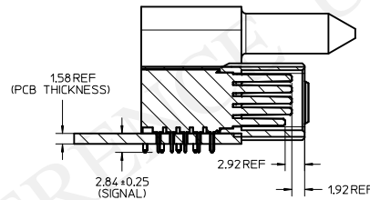
SECTION Z-Z
