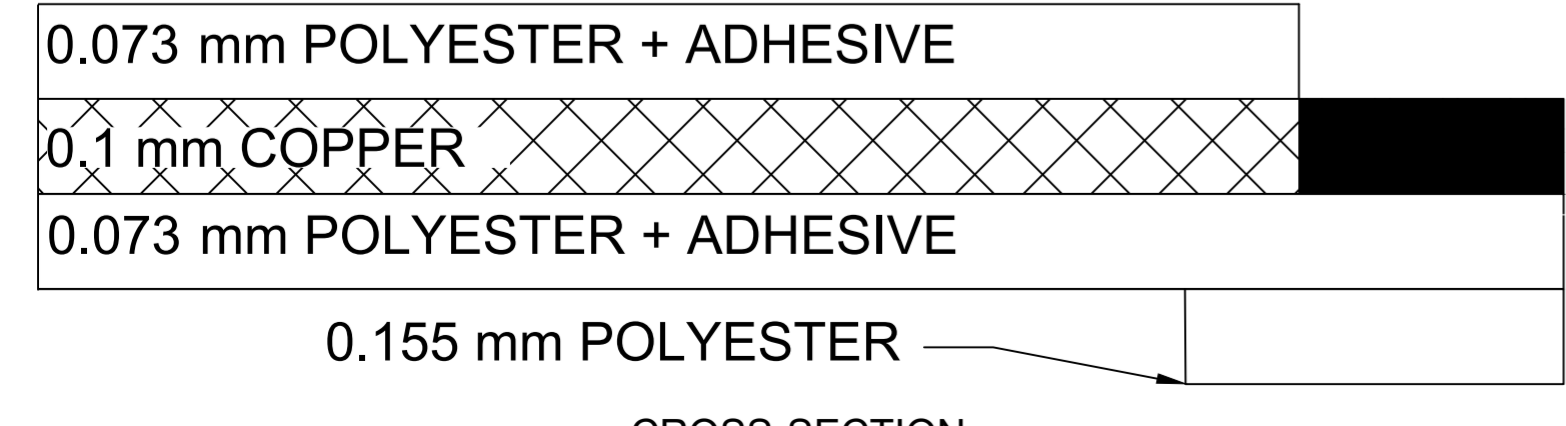
CROSS-SECTION
