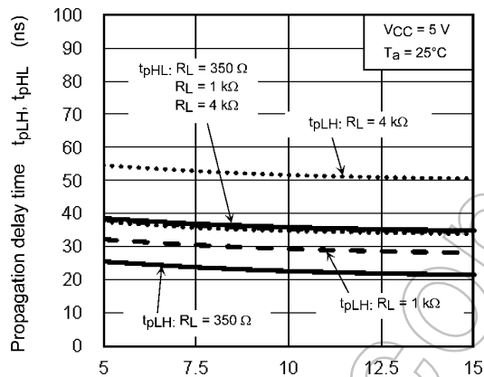
Fig. 12.2.15 t_{pLH}, t_{pHL} - I_F
