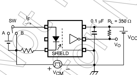
Fig. 12.1.5 Switching Time Test Circuit and Waveform
