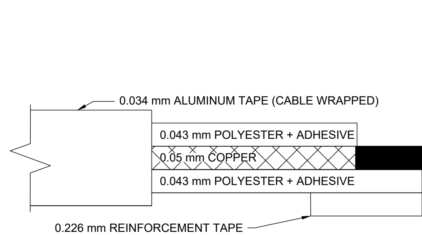
CROSS-SECTION
