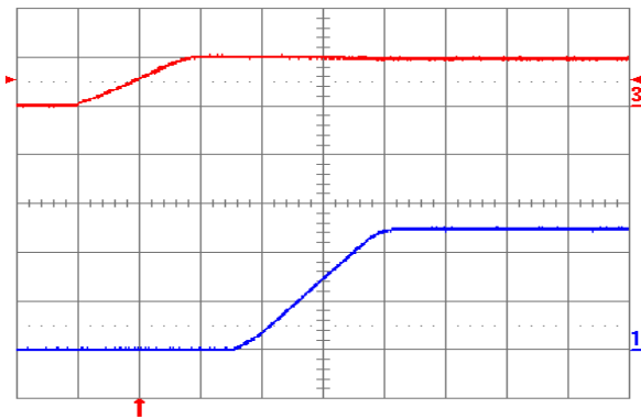
Fig. 2.5V.5: Turn-on transient for V_{out} = 2.5\text{ V} with application of V_{in} at full rated load current (resistive) and 100\text{ }\mu\text{F} external capacitance at V_{in} = 5\text{ V} . Top trace: V_{in} (5 V/div.); Bottom trace: output voltage (1 V/div.); Time scale: 2 ms/div.
