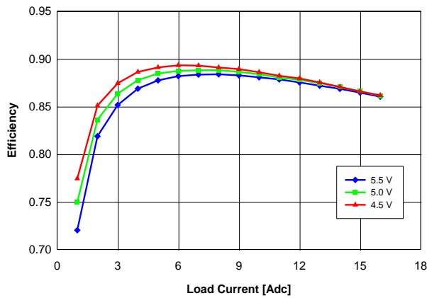
Fig. 1.5V.3: Efficiency vs. load current and input voltage for V_{out} = 1.5\text{ V} converter mounted vertically with air flowing at a rate of 200 LFM (1 m/s) and T_a = 25^\circ\text{C} .
