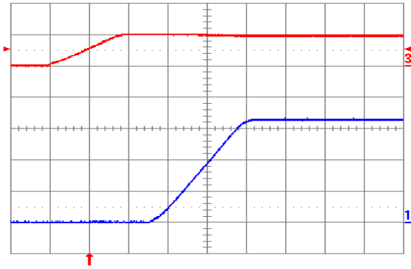
Fig. 3.3V.5: Turn-on transient for V_{out} = 3.3\text{ V} with application of V_{in} at full rated load current (resistive) and 100\text{ }\mu\text{F} external capacitance at V_{in} = 5\text{ V} . Top trace: V_{in} (5 V/div.); Bottom trace: output voltage (1 V/div.); Time scale: 2 ms/div.
