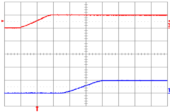
Fig. 1.0V.5: Turn-on transient for V_{out} = 1.0 V with application of V_{in} at full rated load current (resistive) and 100 \mu F external capacitance at V_{in} = 5 V. Top trace: V_{in} (5 V/div.); Bottom trace: output voltage (1 V/div.); Time scale: 2 ms/div.
