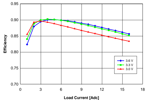
Fig. 1.5V.4: Efficiency vs. load current and input voltage for V_{out} = 1.5\text{ V} converter mounted vertically with air flowing at a rate of 200 LFM (1 m/s) and T_a = 25^\circ\text{C} .
