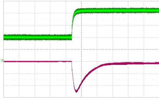
Figure 17. Load transient V_1 , 40 to 85A (500µs/div) CH2: V_1 (200mV/div), CH4: I_1 (20A/div)
