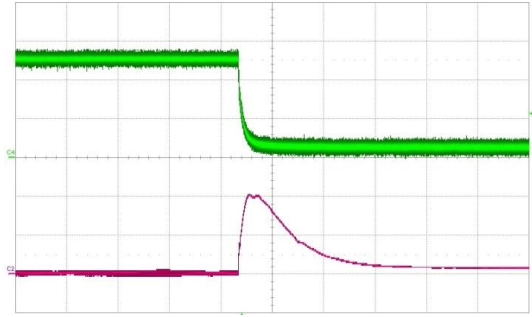
Figure 16. Load transient V 1 , 50 to 5A (500µs/div) CH2: V 1 (200mV/div), CH4: I 1 (20A/div)
