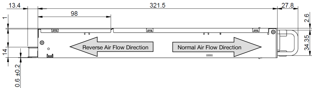
Figure 42. Side View 1
