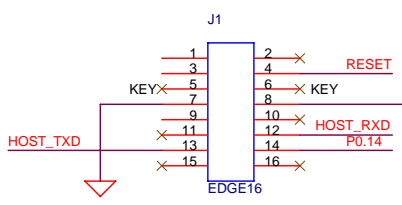
CONNECTOR TO USB-DONGLE
