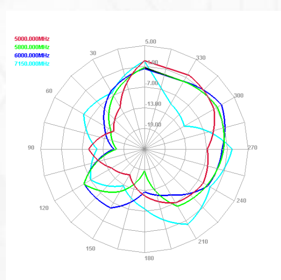
H plane
