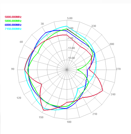
E plane
