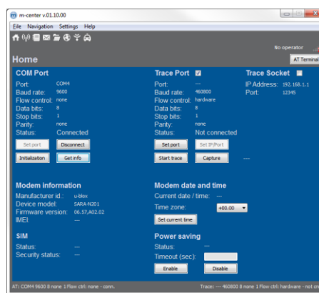
Figure 3: "Home" page
