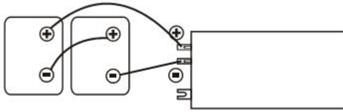
Figure 2: Series battery connection
