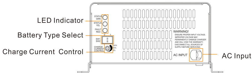
Figure 2 Rear Panel
