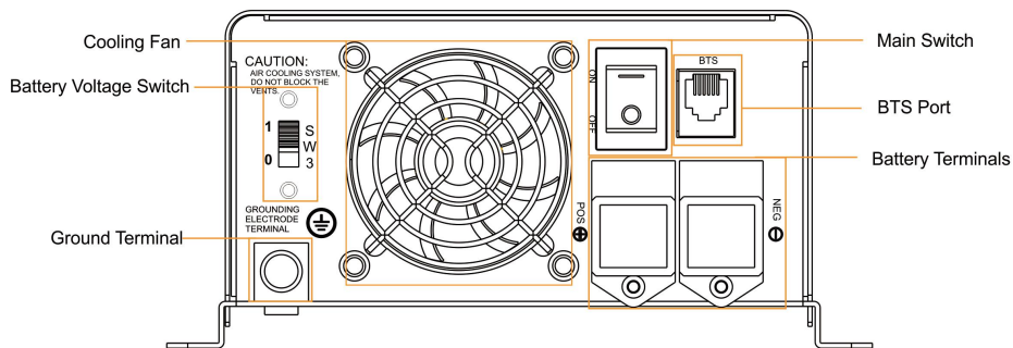
Figure 1 Front Panel
