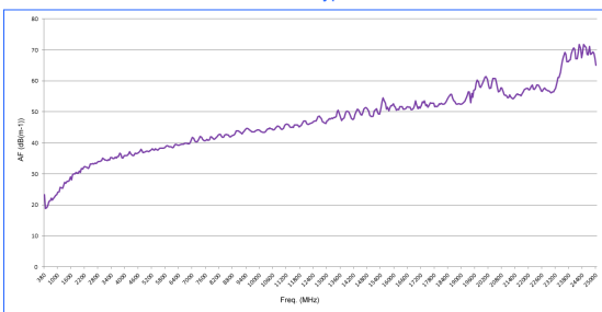
Antenna Factor HyperLOG 30250
