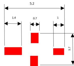
PCB Footprint
