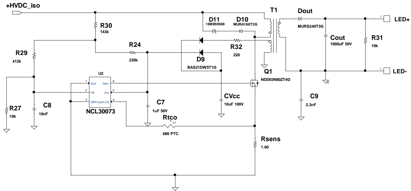
Figure 2. Main Schematic
