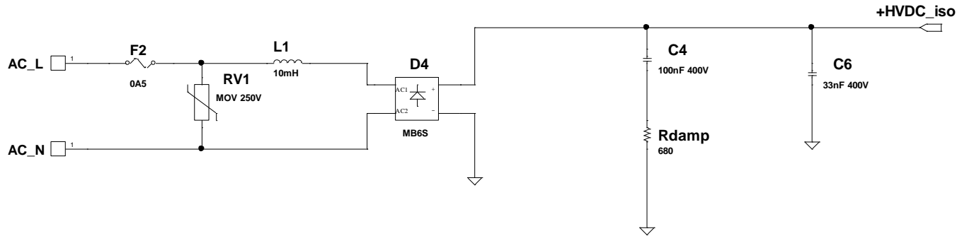
Figure 1. Input Circuit
