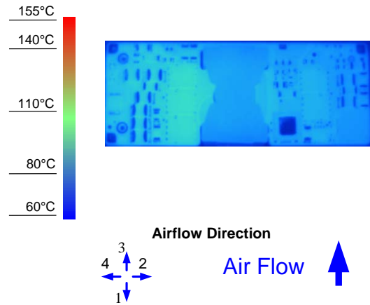
Figure 8. Thermal Image for Airflow Direction 3 (25A output, 55°C ambient, 200 LFM, typical Vin, open frame, socket interface)
