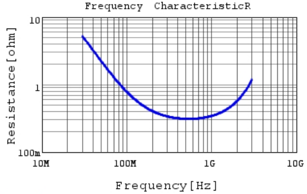
RDE5C2J150J1M1H03A R DC0V, 25degC
