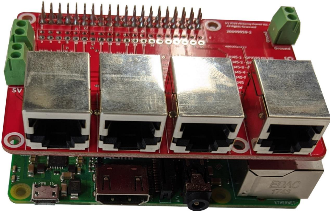
Pi-EzConnect-RJ45 mounted on a Raspberry Pi. Not shown are the spacers to provide mechanical stability to the stack. Raspberry Pi, spacers are not included.
