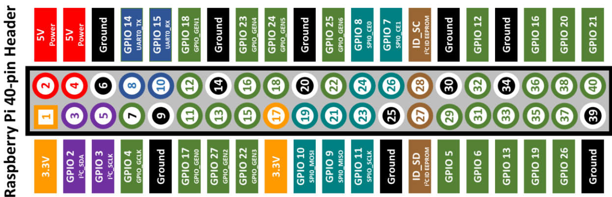
Raspberry Pi 40 pin header definition. Artwork recreated by Alchemy Power Inc.
