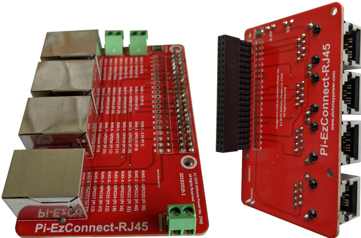
Side view and back view of Pi-EzConnect-RJ45. Note the top layer has the connections documented.
