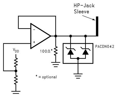
Figure 32. The P4CDN042 provides additional ESD protection beyond the 2000V shown in the Absolute Maximum Ratings for the V O C output
