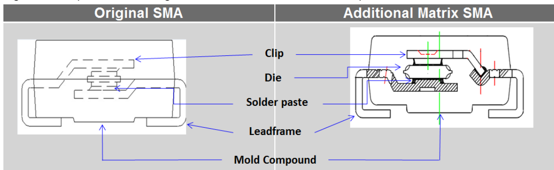
Figure 2: Comparison of Package Construction for Bidirectional TVS products
