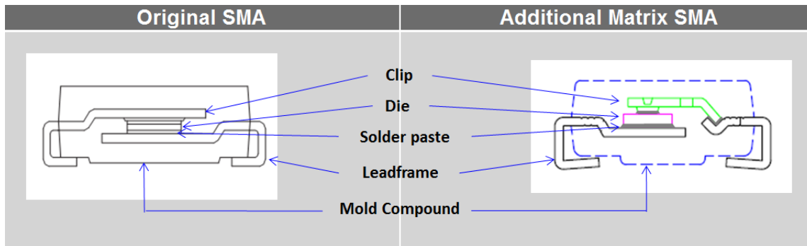
Figure 1: Comparison of Package Construction for Schottky, SBR, GPP Rectifiers, Zener, and Unidirectional TVS products
