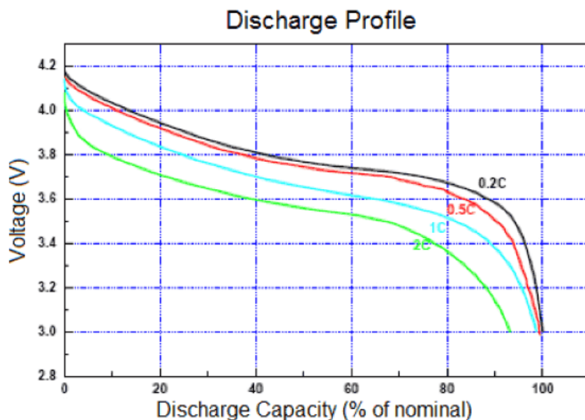
Discharge: 3.0V cutoff at room temperature.
