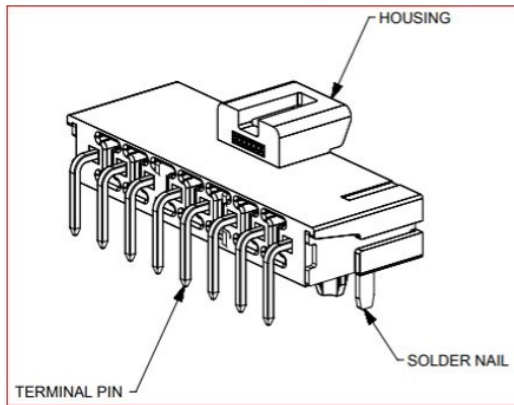
Series 172310 Single Row
