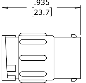
IN-LINE CONNECTOR, MALE MAT'L: NYLON, BLACK
