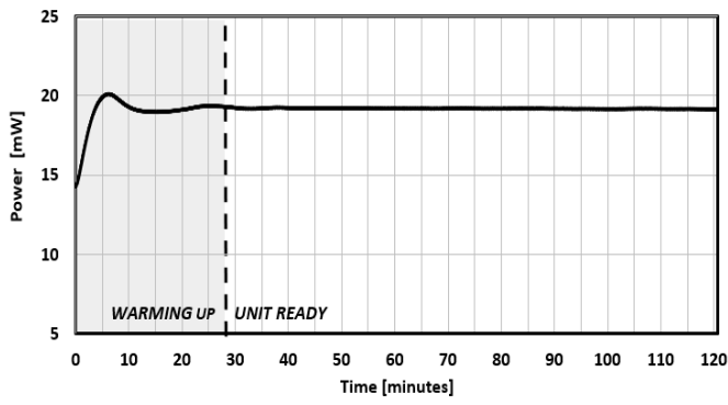
FIG. 9: WARM-UP TIME
