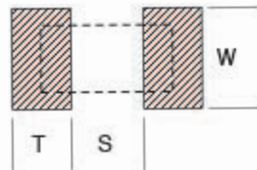
Suggested Landing Patter FR4 copper board, 100µm of copper pad thickness
