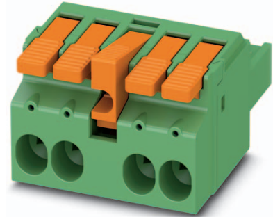
Figure shows a 4-pos. version (GL3 = locking flange on pole 3)
