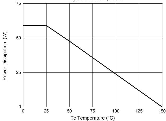
Fig.11-PD Dissipation
