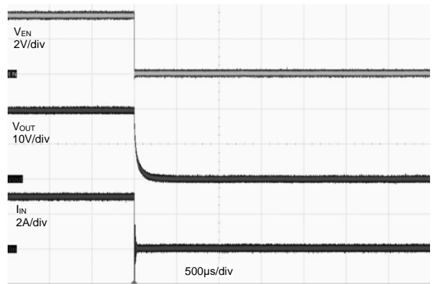
Figure 13. EN Turn OFF V_{IN} = 20\text{V} , Load = 6.7\Omega
