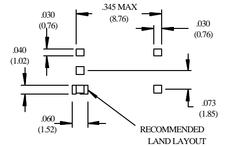
PWB FOOTPRINT
