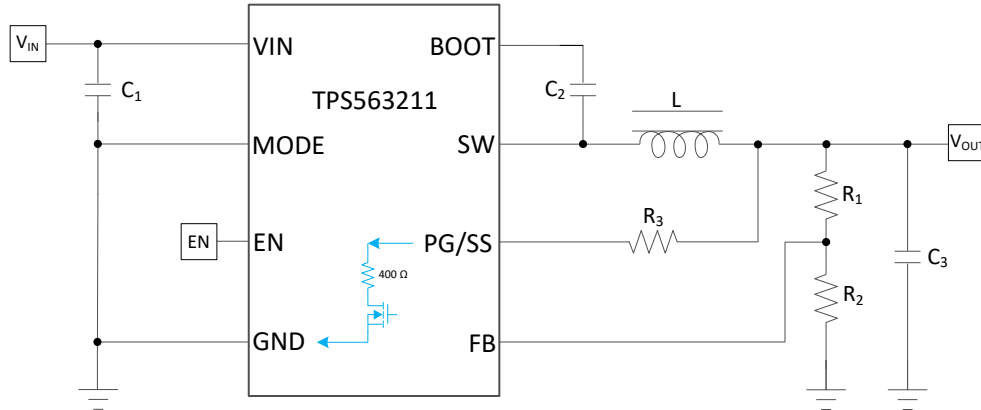
Figure 7-2. Discharge V OUT through PG/SS Pin with TPS563211
