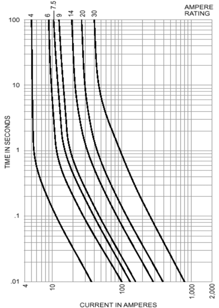
Time-Current Characteristics--Total Clear
