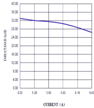
ASPI-1306T-330M
