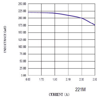
ASPI-1306T-221M
