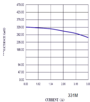
ASPI-1306T-331M
