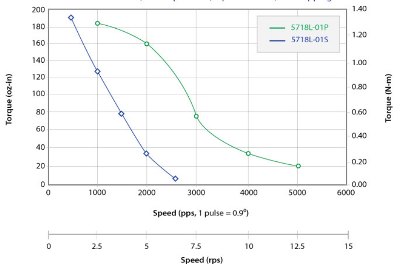
5718L-01S 24VDC, 1.4 Amps/Phase, Bipolar Series, 1/2 Stepping 5718L-01P 24VDC, 2.8 Amps/Phase, Bipolar Parallel, 1/2 Stepping
