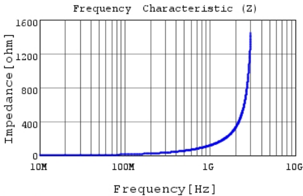
LQG15WZ18NJ02 |Z|
